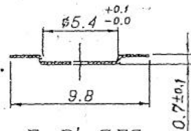
B-B' SEC
