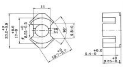
Bobbin for RM8
