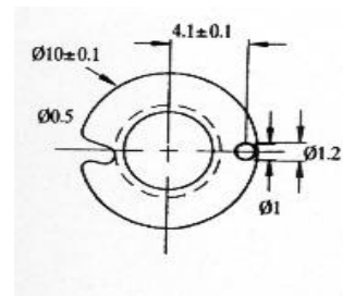
Bobbin for RM5
