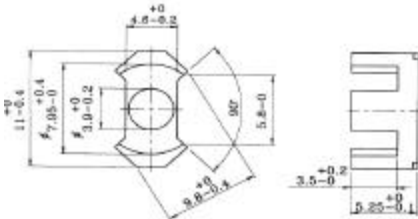
Bobbin for RM4
