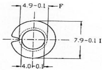
Bobbin for RM4
