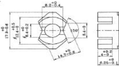
Bobbin for RM6
