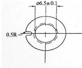
Bobbin for RM6
