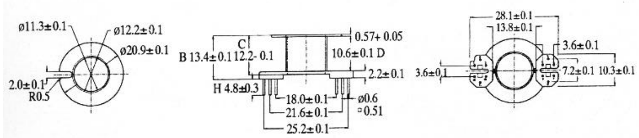
Bobbin for RM10
