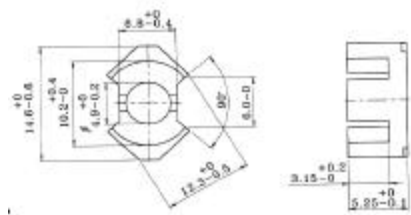
Bobbin for RM5
