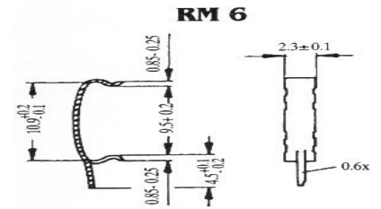
Clamps
