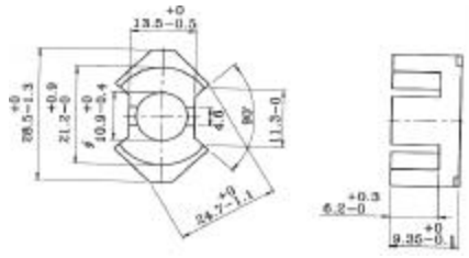
Bobbin for RM10
